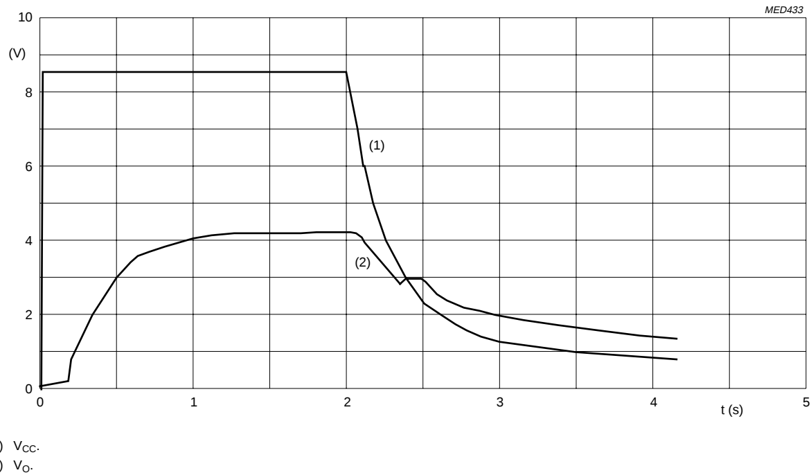
Fig.13 Turn-on/off behaviour.
