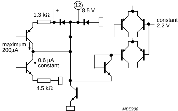
Fig.27 Pin 12: mute control.
