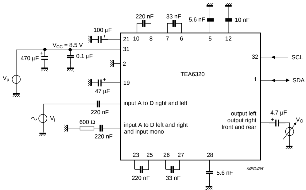
Fig.15 Test circuit for channel separation ( \alpha_{CS} ).
