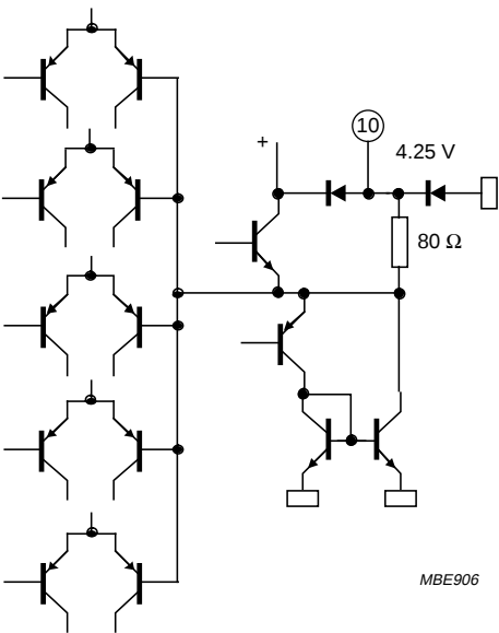
Fig.25 Pins 10 and 23: output source selector.
