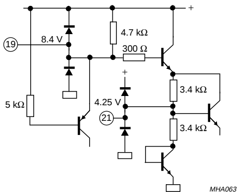
Fig.28 Pin 19: filtering for supply; pin 21: reference voltage.
