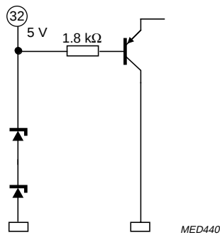
Fig.30 Pin 32: SCL (I2C-bus clock).
